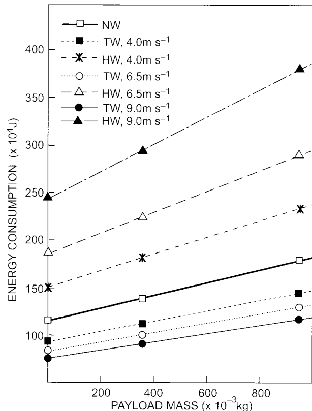
Figure 8: Total energy requirements (calculated from Pennycuik 1989) for a 100km flight by a Cape gannet (mass = 2.63kg, wing span = 1.73m, flight speed = 17.2m s -1 ) carrying payloads ranging from zero, through mean accumulated mass (0.358kg) to the maximum recorded (0.95kg) under various wind conditions (NW: no wind, TW: tailwind, HW: headwind). The most frequently recorded wind speed at Malgas Island was 6.5m s -1
